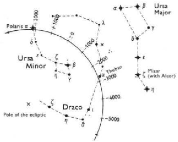
Figure 13. Circumpolar stars and the celestial pole between 5000 BCE and 2000 CE. The semicircle marks the path of the gradually shifting celestial pole. (After Liebert 1969: 168.)
